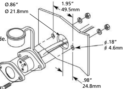
Figure 9 – Socket Assembly mounts from outside/in
